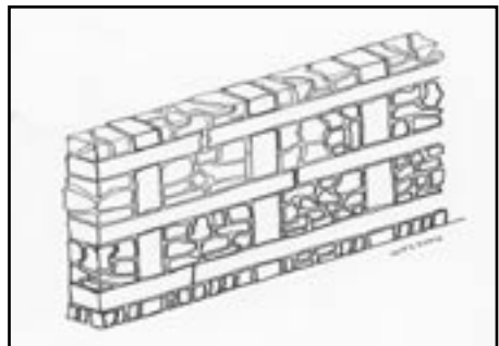
Opus craticium
